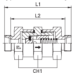
Type: 5001...1 Body
