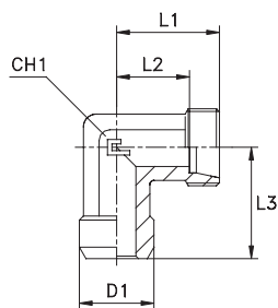
Type: 1058...1 Body
