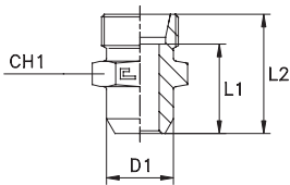
Type: 1055...1 Body
