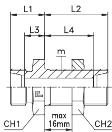
Type: 1036...1 Body
